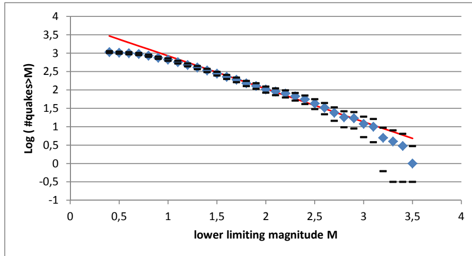
Figure 2.1 The logarithmic cumulative magnitude distribution of earthquakes for all earthquakes in the set. The red line is a linear function with a slope of -1 consistent with the value reported elsewhere ((Dost, B., Goutbeek, F., van Eck, T., Kraaijpoel, D., 2012)). 95% confidence intervals are indicated under the assumption that the underlying process obeys Poisson statistics.
