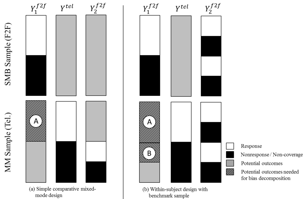
Figure 1: Missing data pattern of a simple comparative mixed-mode design (a) and a within-subject design (b) for estimating bias components against a SMB (Example of a telephone-F2F mixed-mode design with F2F benchmark)
