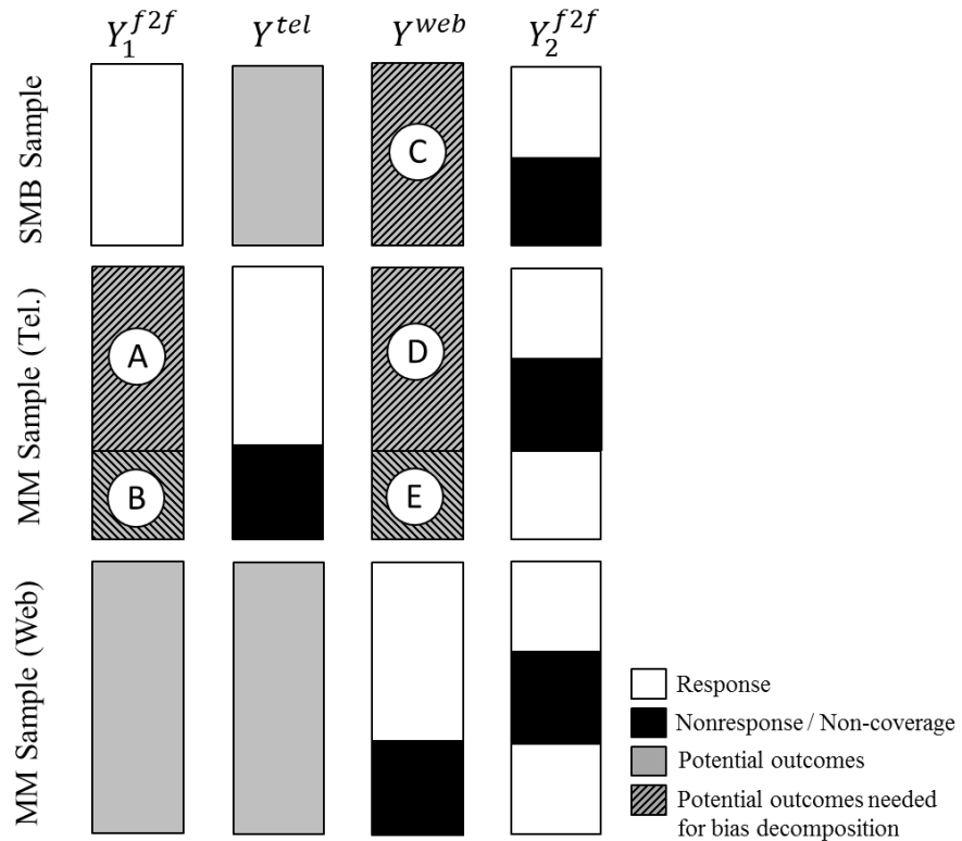
Figure 2: Missing data pattern of an extended within-subject design with two different mixed-mode samples (telephone and web) for use in the HMB case (nonrespondents in the SMB sample and double-nonrespondents in the mixed-mode samples omitted)
