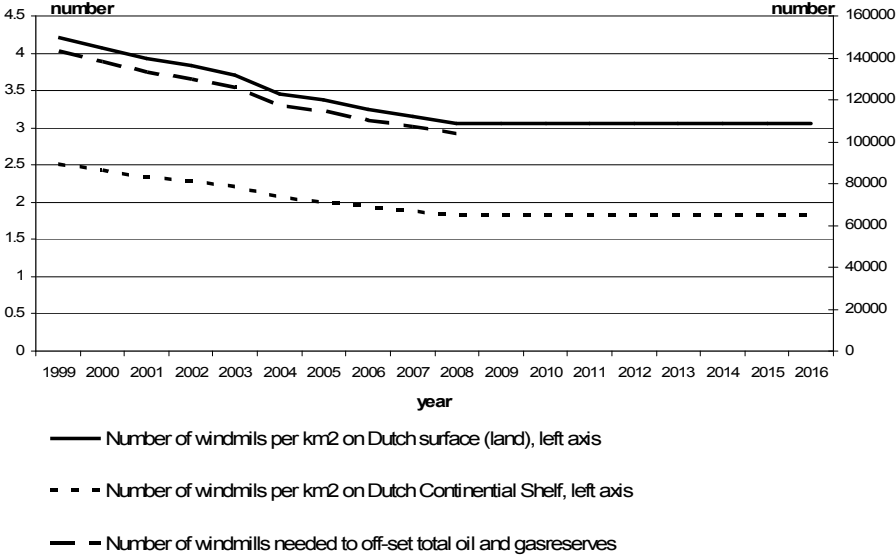
Figure 27- Number of windmills needed to sett-off oil and gas reserves and the scarcity of space
