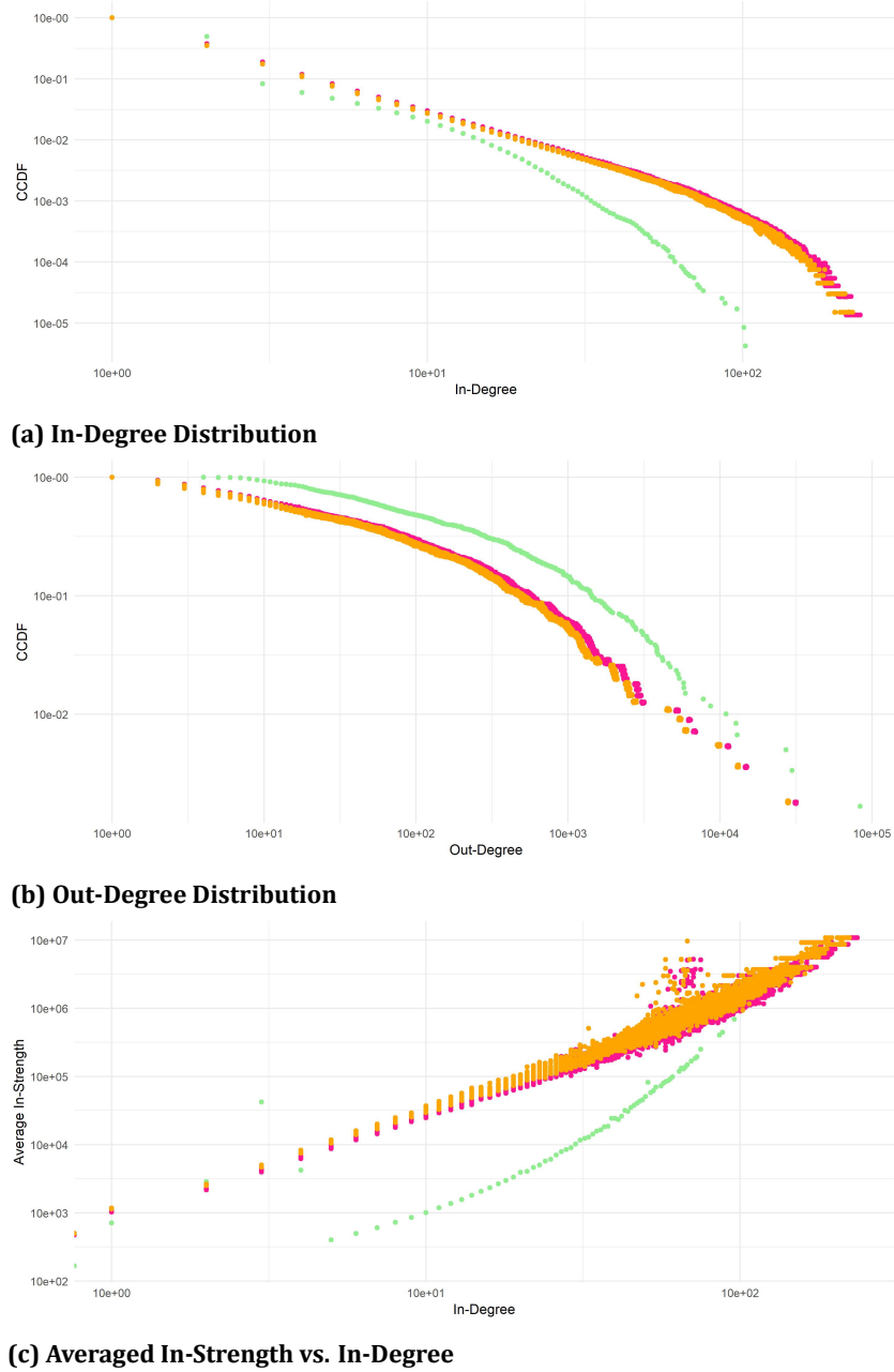
Figure 4.1 Example of Results - Commodity Group 3600000 (Water). Subplots (a), (b), and (c) depicted on the log-log scale. Green line depicts the SN Method, Orange depicts ME Method 1 and Magenta depicts ME Method 2.
