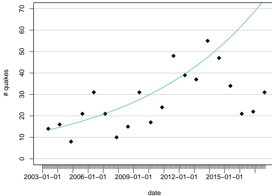
Figure 2.2 The total number of earthquakes for 20 consecutive subsets of equal length time intervals, covering the period from 1 Jan. 2003 to 1 Oct. 2017.
