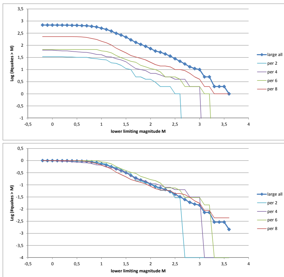
Figure 3 The logarithmic cdf-s of earthquakes for a selection of the 8 consecutive subsets, only every second set is shown for clarity. Upper panel: before normalization, lower panel: after normalization.
