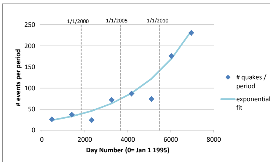
Figure 4 The total number of earthquakes for each of the 8 consecutive subsets and an exponential fit to these points.
